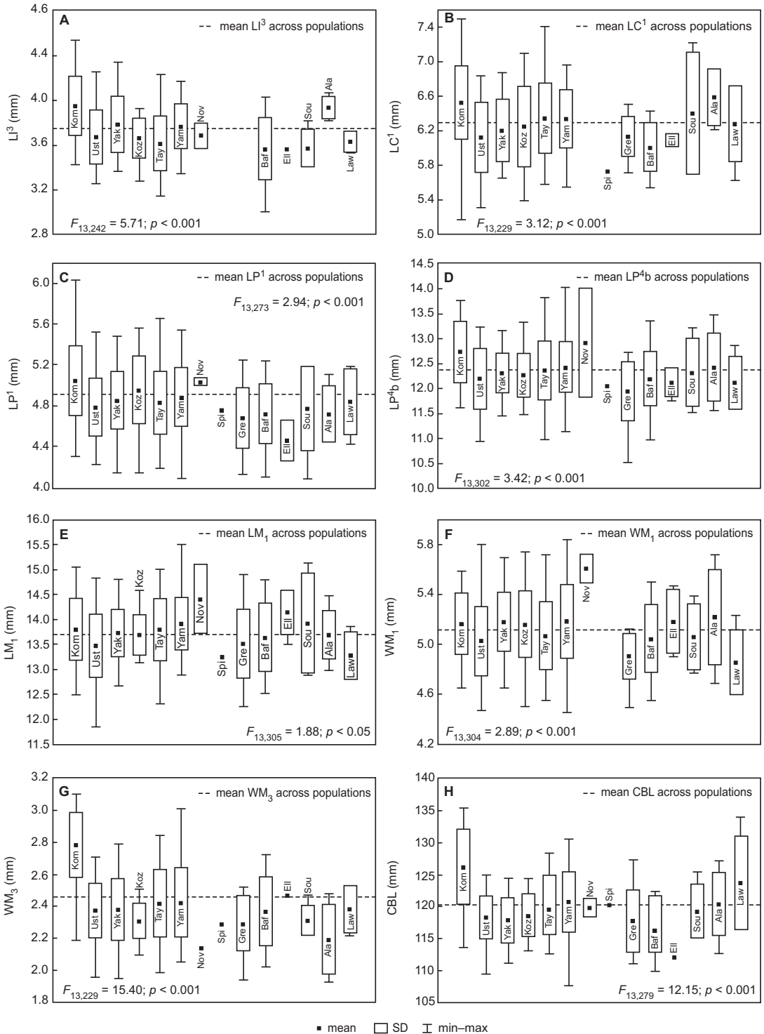
Fig. 2. Variation of (A) length of I^3 – LI^3 ; (B) length of C^1 – LC^1 ; (C) length of P^1 – LP^1 ; (D) buccal length of P^4 – LP^{4b} ; (E) length of M_1 – LM_1 ; (F) width of M_1 – WM_1 ; (G) width of M_3 – WM_3 ; (H) condylobasal skull length (CBL) within geographic range of the arctic fox Vulpes (Alopex) lagopus . Abbreviations as in Fig. 1.
