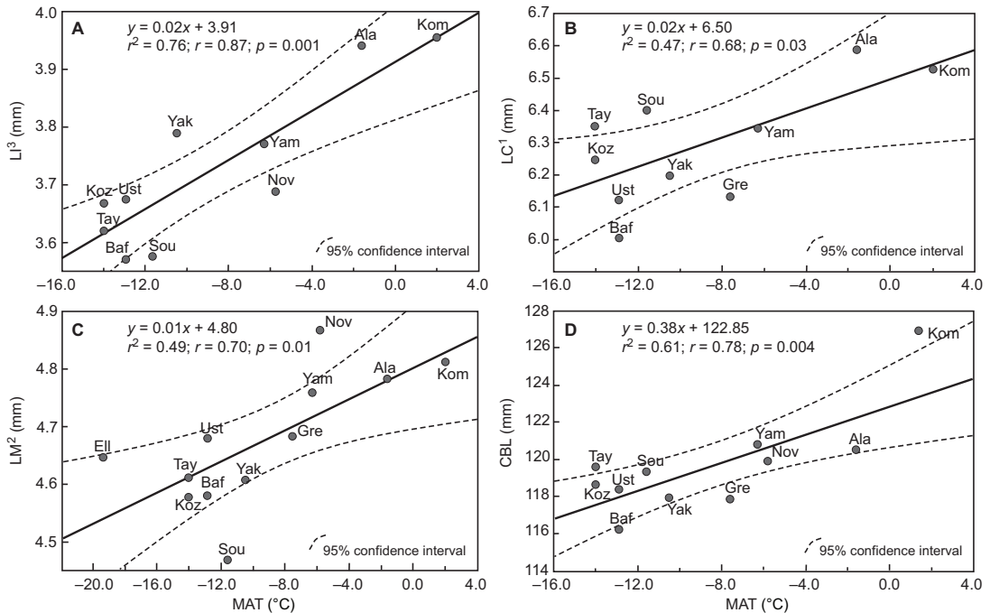
Fig. 5. Relationships between the mean annual temperature, MAT and (A) length of I^3-LI^3 ; (B) length of C^1-LC^1 ; (C) length of M^2-LM^2 ; (D) condylobasal skull length (CBL), in the arctic fox Vulpes (Alopex) lagopus . Abbreviations as in Fig. 1.
