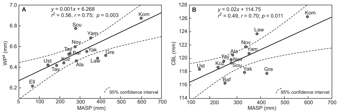
Fig. 6. Relationships between the mean annual precipitation sum (MASP) and (A) width of P^4-WP^4 and (B) condylobasal skull length (CBL), in the arctic fox Vulpes (Alopex) lagopus . Abbreviations as in Fig. 1.
