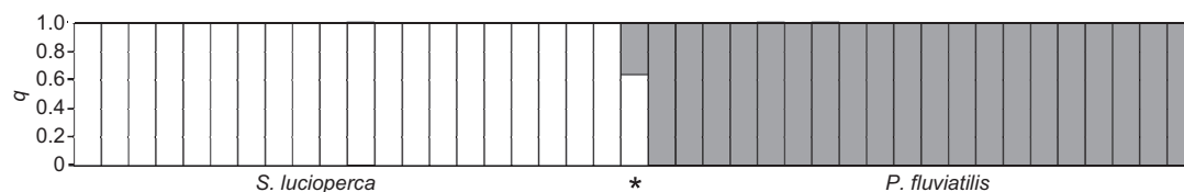
Fig. 1. Genetic assignment ( q ) of the S. lucioperca backcross (marked with a star) to reference species (white = S. lucioperca , grey = P. fluviatilis ) using STRUCTURE. Each vertical column represents one individual.
