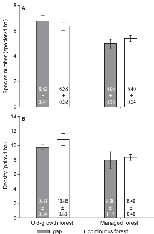
Fig. 1. (A) Mean \pm SE number of species, and (B) total \pm SE density of breeding birds per 4 ha in gaps and continuous forest in the old-growth and managed forests. Mean \pm SE values are also shown in the columns.
